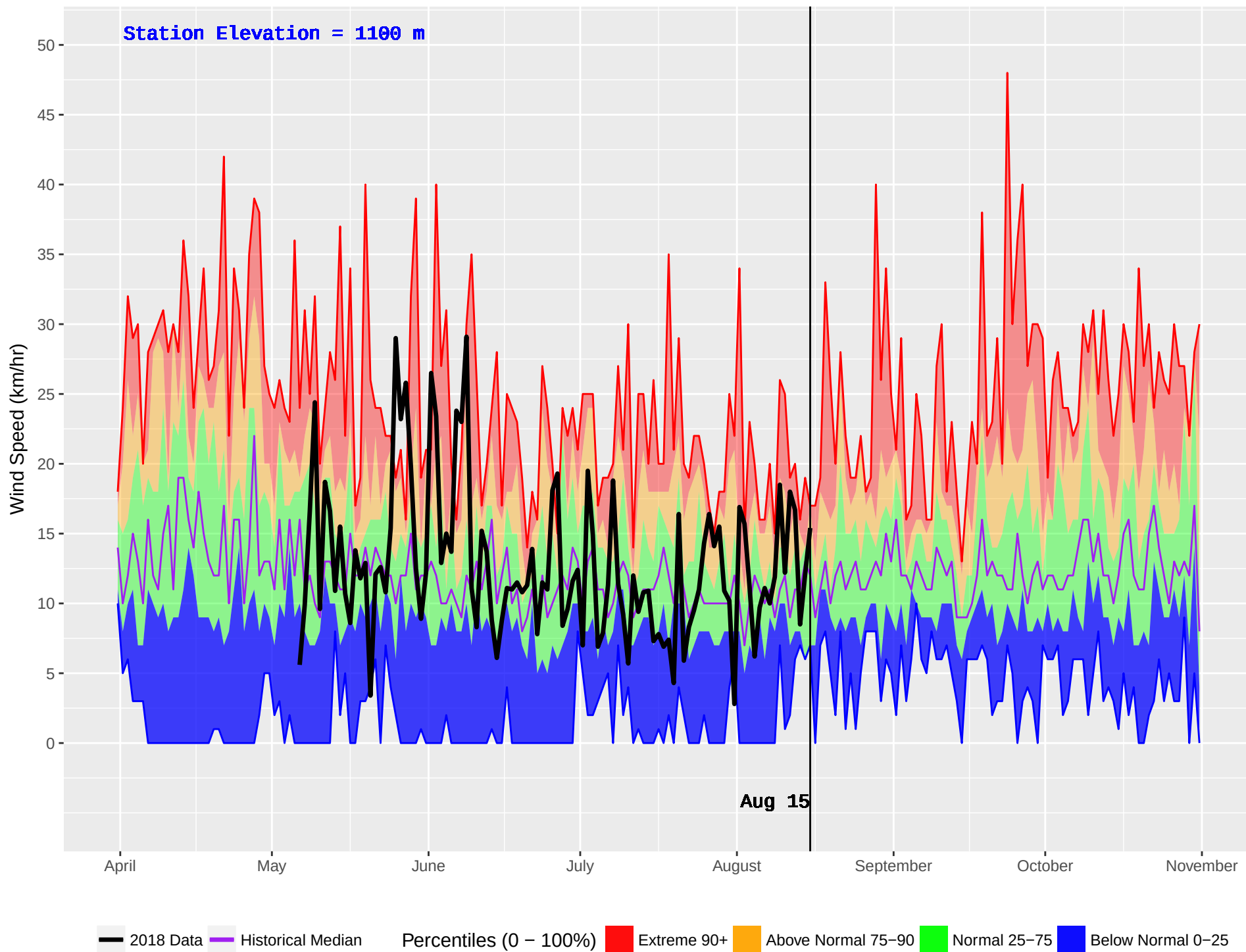
CHURN CREEK (832) : Historical (2003–2016) and Current (2018) Daily Wind Speed
